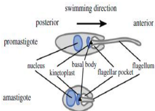
FIGURE 3. shown Promastigote & Amastigote phases [26]
